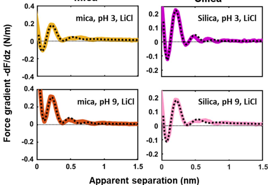
Fig. 6 Averaged ( n = 100 ) force gradient ( -dF/dz ; colored thick lines) versus apparent tip-sample separation measured in 50 mM LiCl solutions, with bulk pH values of pH 3 and 9, on a silica and mica substrate. The pH was adjusted by adding either HCl or NaOH. The data shown here were collected using the same AFM probe. The dotted lines represent the fit using eqn (1).
