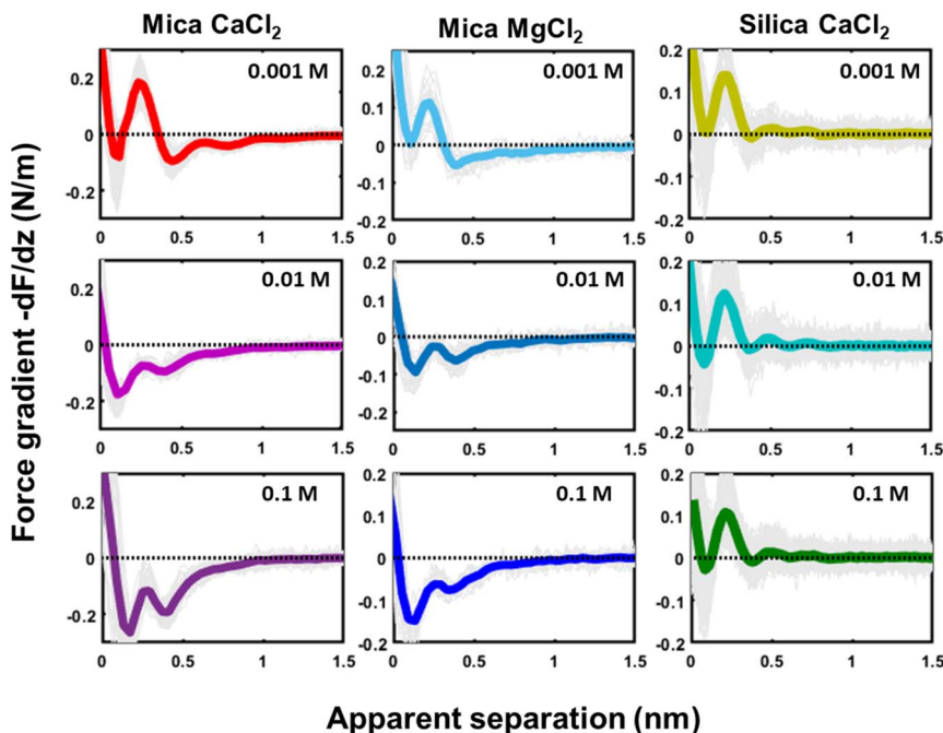
Fig. 4 Force gradient ( -dF/dz (N m -1 ) versus apparent separation (nm) measured in 1, 10 and 100 mM of CaCl 2 and MgCl 2 on a mica substrate and of CaCl 2 on a silica substrate. The thin gray lines are individual measured curves, the thick line is the average of these lines. The measurements at the mica and silica substrate are obtained with different tips at pH 6.
