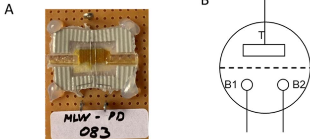
Fig. 1 (A) Device construction. (B) Device symbol.
