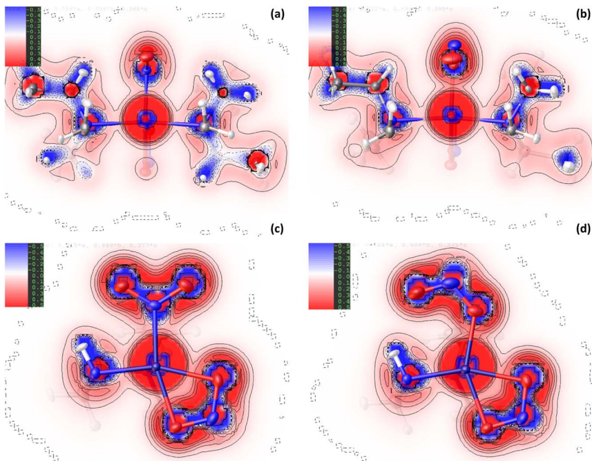
Fig. 5 2D Laplacian maps for the ground state (GS) and excited state (ES) of complex 2, produced by HAR using NoSpherA2, showing regions of charge concentration (blue = negative values of \nabla^2\rho(r) ) and charge depletion (red = positive values of \nabla^2\rho(r) ). (a) GS map in the Ni(1), N(1), N(3), N(5) plane, (b) ES map in the Ni(1), O(1A), N(3), N(5) plane, (c) GS map in the Ni(1), N(1), O(1), O(2) plane (plane of the nitro ligand), (d) ES map in the Ni(1), N(1A), O(1A), O(2A) plane (plane of the nitrito ligand).
