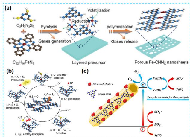
Fig. 32 (a) Fabrication scheme of Fe-CNN x . (b) Catalytic reaction mechanism of H 2 S selective oxidation on Fe-CNN x . (c) Schematic illustration of mechanisms for S(IV) activation by MF 2 under visible light irradiation. 70
