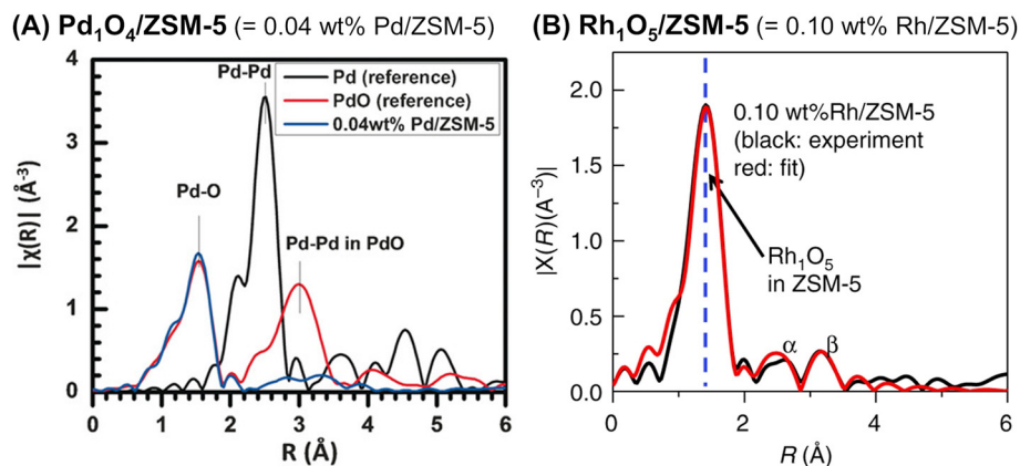
Fig. 21 Fourier transform of EXAFS spectra of (A) \text{Pd}_1\text{O}_4/\text{ZSM-5} ( k^2 -weighted Pd K-edge) and (B) \text{Rh}_1\text{O}_5/\text{ZSM-5} ( k^2 -weighted Rh K-edge). Reprinted from (A) ref. 81 with permission from John Wiley and Sons, copyright 2016, and (B) ref. 82 with permission from Springer Nature, copyright 2018.
