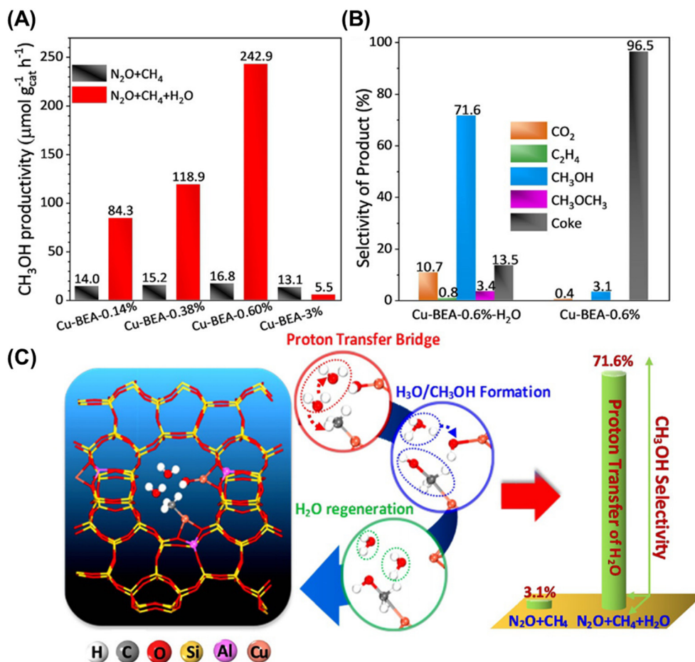
Fig. 12 (A) Methanol productivity of Cu-BEAs for methane to methanol reaction in the presence (red) and absence (black) of \text{H}_2\text{O} . Reaction conditions: \text{N}_2\text{O} : \text{CH}_4 : \text{H}_2\text{O} : \text{He} = 30 : 15 : 10(0) : 45(55) ; GHSV = 12\,000 \text{ h}^{-1} ; 593 K; TOS = 6 h. (B) Selectivity of products over Cu-BEA under the same reaction conditions as figure A, TOS = 70 h. (C) Schematic of high-speed proton transfer bridge between the generated \text{CH}_3^- and \text{OH}^- moieties. Reprinted from ref. 52 with permission from John Wiley and Sons, copyright 2021.
