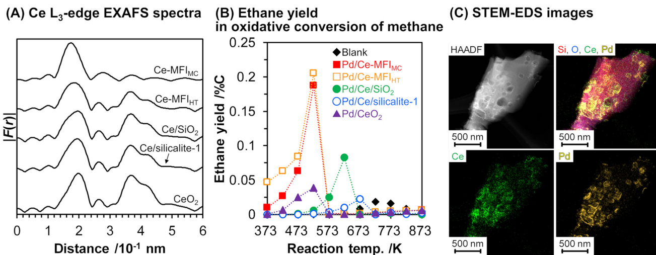
Fig. 22 (A) Fourier transform of k^3 -weighted Ce L_3 -edge EXAFS spectra for Ce-containing supports, (B) ethane yield in oxidative conversion of methane over 3 wt% \text{Pd}/\text{support} , and (C) STEM-EDS images of 3 wt% \text{Pd}/\text{Ce-MFI}_{\text{MC}} . Reaction conditions: \text{CH}_4/\text{O}_2/\text{Ar}_2 = 8.0/2.0/2.5 mL \text{min}^{-1} ; \text{SV} = 7.5 \times 10^3 mL \text{g}_{\text{cat}}^{-1} \text{h}^{-1} ; 373–873 K; 0.1 MPa. Reproduced from ref. 85 with permission from American Chemical Society, copyright 2021.
