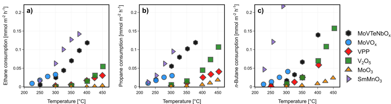
Fig. 1 Catalytic activity of \text{MoVTenbO}_x , \text{MoVO}_x , \text{MoO}_3 , \text{V}_2\text{O}_5 , VPP and \text{SmMnO}_3 : alkane consumption rates normalized to the surface area [ \text{mmol m}^{-2} \text{h}^{-1} ] as a function of the reaction temperature in (a) ethane, (b) propane, and (c) n -butane oxidation; the corresponding alkane conversions and consumption rates normalized to weight can be found in Fig. S13;† oxygen consumption rates are shown in Fig. S14;† \text{C}_2\text{H}_6/\text{O}_2/\text{H}_2\text{O} = 3/9/0 % vol, \text{C}_3\text{H}_8/\text{O}_2/\text{H}_2\text{O} = 3/9/20 % vol, \text{C}_4\text{H}_{10}/\text{O}_2/\text{H}_2\text{O} = 2/20/3 % vol, 1 atm, 1000 \text{ h}^{-1} ( \text{C}_2 , \text{C}_3 )/ 2000 \text{ h}^{-1} ( \text{C}_4 ).
