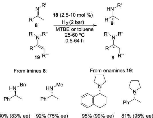
Scheme 8 Asymmetric hydrogenation of imines and enamines with ansa -ammonium borate catalysts.
