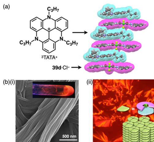
Fig. 27 (a) Single-crystal X-ray structure of {}^3\text{TATA}^+-\mathbf{39d}\cdot\text{Cl}^- (redrawn from a cif file: 745780) and (b) (i) photograph and SEM of the supramolecular gel and (ii) POM and packing model of the liquid crystal mesophase of {}^3\text{TATA}^+-\mathbf{39e}\cdot\text{Cl}^- (redrawn from ref. 7. Copyright 2010 Wiley).
