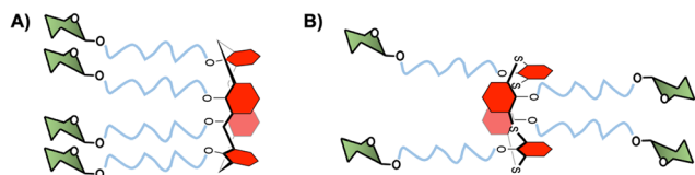
Fig. 4 (A) Cone conformation of the glycolix[4]arenes, and (B) 1,3-alternate conformation of glycolix[4]arenes.
