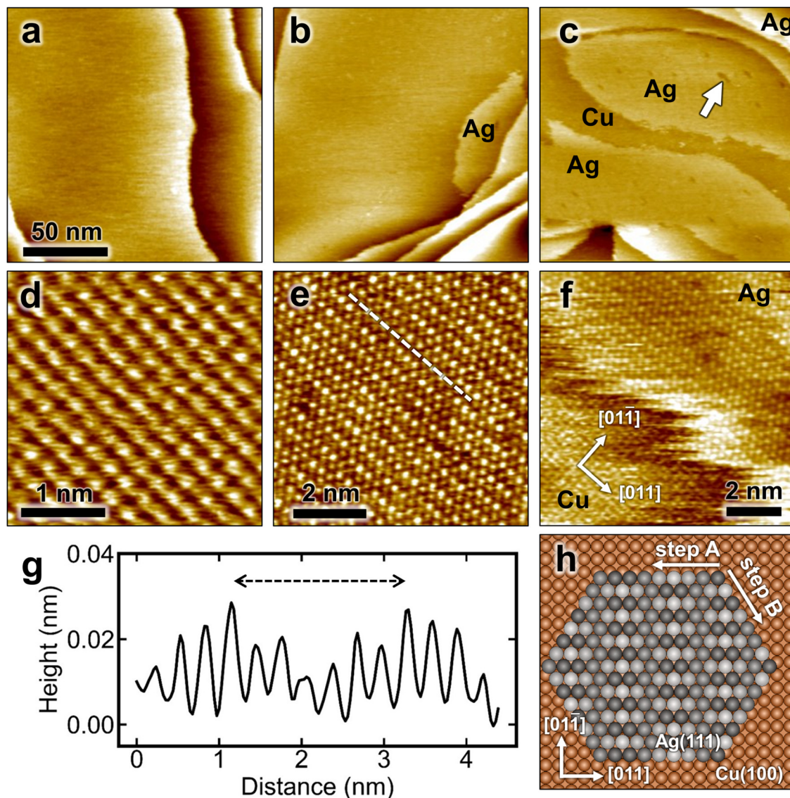
Fig. 1 In situ STM images of Cu(100) surface (a) before and (b) and (c) after 0.1 ML and 0.7 ML Ag deposition at (b) 0.05 and (c) -0.04 V in 0.1 M H 2 SO 4 . (d)–(f) Atomic-resolution images of (d) the Cu(100) substrate lattice, (e) the atomic structure of the Ag islands, revealing a quasi-hexagonal structure with a long range modulation, and (f) the border between the Cu substrate and an Ag island (recorded at -0.04 V). The image in (f) shows that the Ag atomic rows along the direction of the long-range modulation are aligned with one of the close-packed directions of the underlying Cu lattice. (g) Apparent height profile along the white dashed line in (e), illustrating the long-range modulation of the Ag-decorated Cu(100). (h) Atomic model of Ag-adlayer, showing the corresponding modulation due to the different adsorption position of Ag on Cu(100). Different gray scales demonstrate the change of the apparent height in the STM images.
