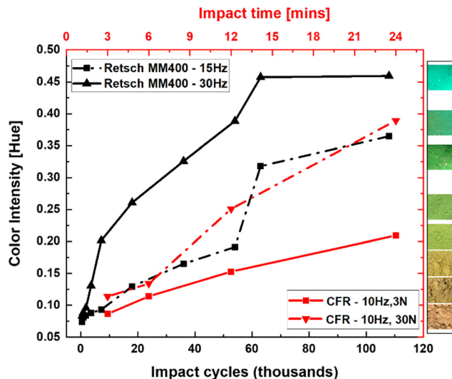
Fig. 7 Reaction of copper(II) chloride anhydrous and 1,10-phenanthroline with color intensity measured at different force levels and impact cycles using the controlled force reactor and the Retsch MM400 ball mill reactor. Images of products taken after reaction are placed on the right next to the reaction timestamp.
