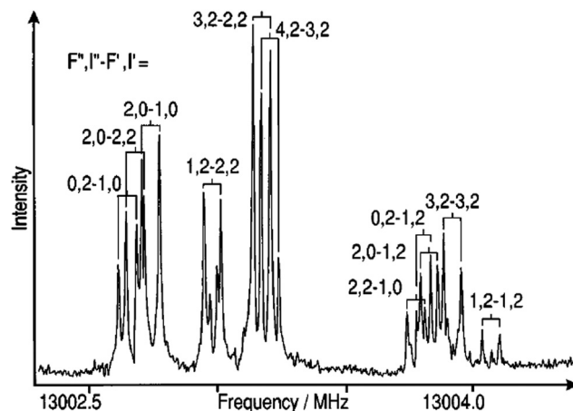
Fig. 1 A composite spectrum of the J_{Ka,Kc} = 20,2 - 10,1 rotational transition of ^{20}\text{Ne}-^{14}\text{N}_2 van der Waals complex showing complicated nuclear hyperfine structure due to the ^{14}\text{N} nuclei. 3 The missing rotational transitions were recovered from the new measurements guided by CMS.
