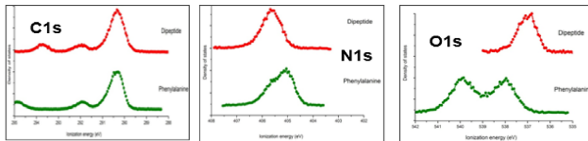
Fig. 9 (a) The CMS simulated C1s, N1s and O1s spectra of phenylalanine monomer and linear phenylalanyl–phenylalanine (dipeptide) and (b) the actually measured XPS spectra. 62
