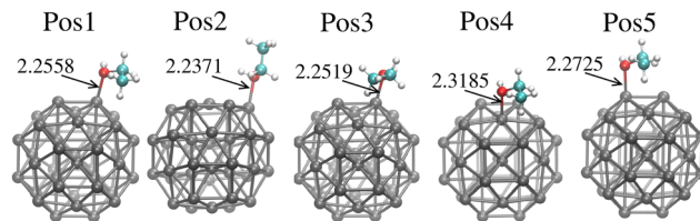
Fig. 1 Ethanol adsorption sites on Pt 38 nanoparticles. Each position shows the distance between ethanol–oxygen and Pt-anchors in Å units. Grey, cyan, white and red balls represent the Pt, C, H, and O atoms, respectively.
