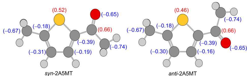
Fig. 7 Charge distribution in syn - and anti -2A5MT obtained from NBO calculations at the MP2/6-31G(d,p) level of theory.
