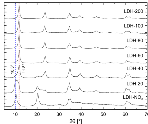
Fig. 1 PXRD patterns of pristine \text{LDH-NO}_3^- and the anion exchanged samples \text{LDH-A} ( A = 20, 40, 60, 80, 100 and 200 standing for the initial carbonate concentration in \text{mmol L}^{-1} in the anion exchange solution). The \text{NO}_3^- - and \text{CO}_3^{2-} -intercalated phases can be identified by the characteristic basal reflections at 10.3^\circ and 11.8^\circ 2\theta , respectively.
