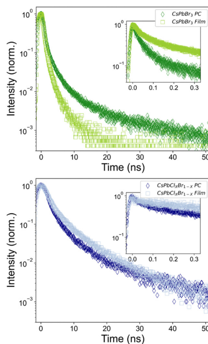
Fig. 3 Time-resolved photoluminescence (TRPL) dynamics of neat PNC films and PC <math>C</math>PNCs. PL decay traces of: (A) CsPbBr 3 NCs ( \lambda_{\text{ex}} = 390 nm). (B) CsPbCl 1.5 Br 1.5 NCs ( \lambda_{\text{ex}} = 350 nm).
