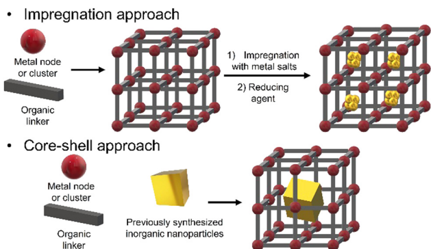
Fig. 5 Schematic representation of different approaches to produce inPNs@NMOFs nanocomposites.
