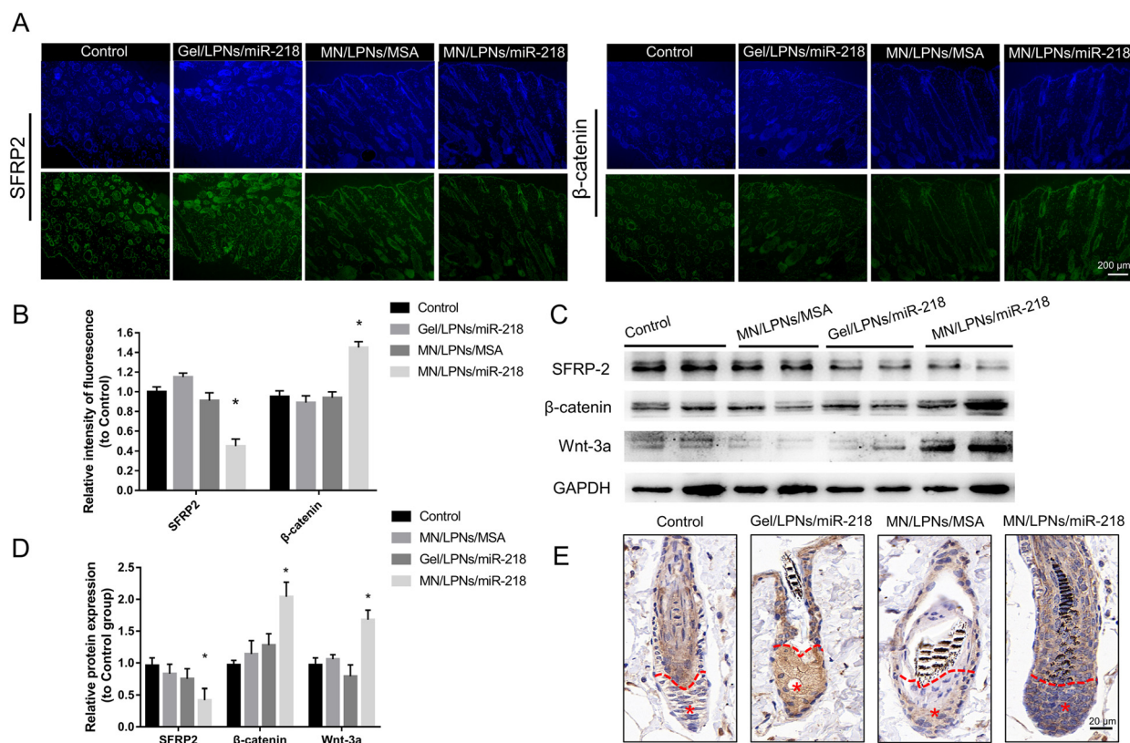
Fig. 6 In vivo evaluation of the regulation of MN/LPNs-miR-218 on Wnt/β-catenin channel. (A) Immunofluorescence of β-catenin and SFRP2 on the skin after 13 days of treatment (scale bars = 200 μm). (B) Statistical result of fluorescence intensity. (C) Western blot and (D) statistical result of Wnt/β-catenin channel markers and miR-218 target gene in the skin after 13 days treatment, * P < 0.05 vs. Gel/LPNs/miR-218. (E) Immunohistochemical of versican on the skin after 13 days treatment (*: DP aggregates, scale bars = 20 μm). Data were shown as mean \pm SD ( n = 5 ), and statistical significance was calculated by one-way ANOVA followed by Dunnett's test.
