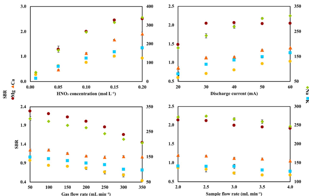
Fig. 2 The impact of \text{HNO}_3 concentration, discharge current, gas flow rate, and sample flow rate on the SBR values of the analytical lines of the studied elements for a solution containing only the analytes.
