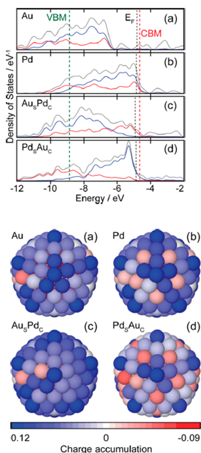
Fig. 22 (a–d) Electronic density of states (DOS) profiles of 147-atom icosahedral clusters of Au, Pd, Au 8 Pd C , and Pd 8 Au C , respectively. The total valence DOS (gray) is complemented by the contributions of the d-orbitals in both the core (red) and outer shell (blue) region. E_F of the metal clusters, conduction band minima (CBM), and valence band maxima (VBM) of TiO 2 are indicated by black and red dashed lines, respectively. 261 27B (a–d) Charge localization from the view of the (100) surface of 147-atom icosahedral clusters of Au, Pd, Au 8 Pd C , and Pd 8 Au C , respectively. The blue and red colors represent atoms with electron accumulation and depletion, respectively. Reprinted with permission from American Chemical Society. 177
