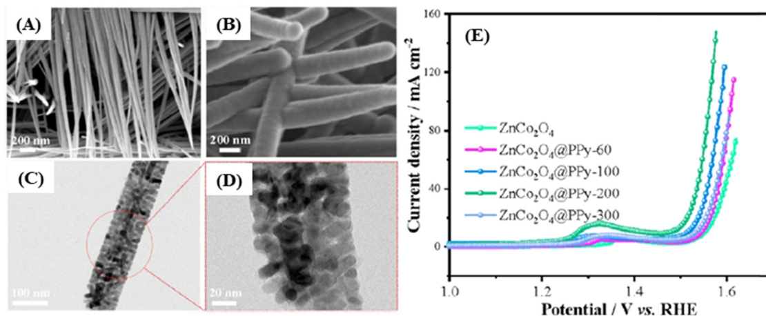
Fig. 21 SEM images of \text{ZnCo}_2\text{O}_4 (A) and \text{ZnCo}_2\text{O}_4@\text{PPy-200} (B). TEM images of \text{ZnCo}_2\text{O}_4@\text{PPy-200} (C and D). Linear sweep voltammetry at 2 \text{ mV s}^{-1} for \text{ZnCo}_2\text{O}_4 and \text{ZnCo}_2\text{O}_4@\text{PPy} samples (E). Reproduced with permission. 275 Copyright © 2021 Elsevier Ltd. All rights reserved.
