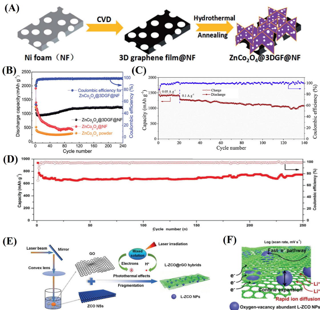
Fig. 16 (A) Schematic illustration of the synthesis of \text{ZnCo}_2\text{O}_4@3\text{D} graphene foam@nickel foam composites. (B) Comparison of cycle performance of the \text{ZnCo}_2\text{O}_4@3\text{DGF@NF} , \text{ZnCo}_2\text{O}_4@NF , and \text{ZnCo}_2\text{O}_4 powder electrodes at a current density of 500 \text{ mA g}^{-1} . Reproduced with permission. 191 CC BY-NC 3.0. Royal Society of Chemistry. (C) Cycling capacity of the ZCO@rGO//LiCoO 2 full cell at a current density of 100 \text{ mA g}^{-1} . Reproduced with permission. 188 Copyright © 2018 Elsevier Ltd. All rights reserved. (D) Cycling performance and coulombic efficiency data at 1.0 \text{ A g}^{-1} of L-ZCO@rGO-30. (E) The schematic diagram for the formation of L-ZCO@rGO hybrids. (F) Schematic illustration of the fast electron/ion transfer and rapid electrochemical kinetics of the L-ZCO@rGO-30 electrode. Reproduced with permission. 192 Copyright © 2020 Wiley-VCH Verlag GmbH & Co. KGaA, Weinheim.
