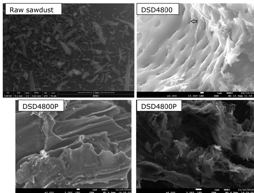
Fig. 1 SEM images of raw sawdust and selected activated and compactivated carbons.
