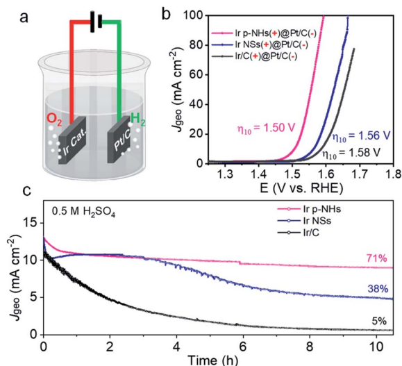
Fig. 4 Initial electrocatalytic overall water splitting performance in 0.5\text{ M H}_2\text{SO}_4 . (a) Scheme of the two-electrode cell electrolyzer using the Ir-based catalyst as the anode and 20% Pt/C as the cathode. (b) Polarization curves of Ir p-NHs, Ir NSs and Ir/C for overall water splitting. (c) Durability test for the three catalysts in a two-electrode configuration.
