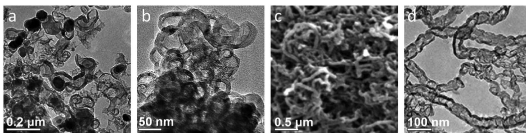
Fig. 6 TEM images of (a) graphitic nanostructures with embedded iron nanoparticles produced by pyrolyzing a mixture of sucrose and iron nitrate and (b) the same sample after acid-washing. (c) Scanning electron microscope (SEM) and (d) TEM images of graphitic nanotubes produced from glucose and iron nitrate (after acid washing to remove iron catalyst particles). Figures modified with permission from ref. 99 and 100.
