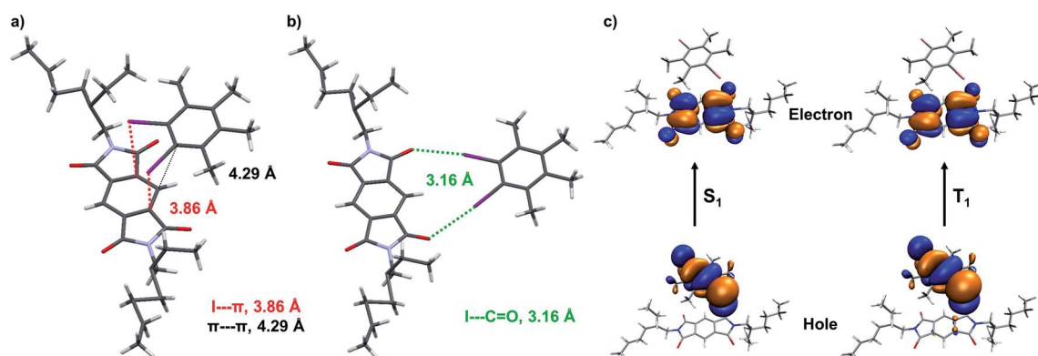
Fig. 4 (a) Single-crystal X-ray diffraction data of A+D 2 co-crystal: donor–acceptor arrangement of A+D 2 pair, driven by various halogen bonding and weak \pi ... \pi interactions, such as (a) I... \pi (marked with red lines), \pi ... \pi (marked with black lines) in a stack and (b) I...C=O (marked with green lines) in the same plane. (c) Theoretical calculations of A+D 1 : natural transition orbitals (NTOs) of A+D 1 pair for first excited singlet (S 1 ) and triplet state (T 1 ), calculated using TD-CAM-B3LYP level in conjunction with 6-31+g(d) basis set for C, N, O, H and LANL2DZ basis set showing CT character.
