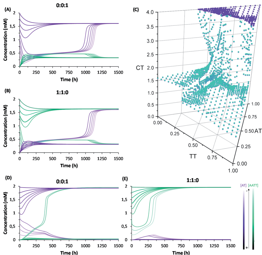
Fig. 4 Simulations of the network evolution when fed with two input streams ( Q_{in} = 1 \mu\text{L min}^{-1} ) of A and T, in the presence of replicator AT (0–2 mM) (A) or AA/TT (0–2 mM) (B). (C) 3D surface representing the reached steady state (SS AT below the surface; SS AA/TT above) for a range of initial replicator proportions (horizontal axes on the graph) and total replicator concentrations (CT, vertical axis). The surface marks the boundary between initial conditions that favour SS AT (below the surface) or SS AA/TT (above). (D, E) Simulations of the network evolution when decreasing the exchange constants by six orders of magnitude, with the same input streams and conditions as in (A) and (B).
