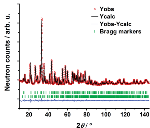
Fig. 1 Rietveld refinement of \text{Cs}_3\text{MoO}_4\text{D} based on powder neutron diffraction. Bragg markers: \text{Cs}_3\text{MoO}_4\text{D} (top) (90.3(10) wt%); \text{CsD} (bottom) (9.7(1) wt%). R_p = 1.18\% , R_{wp} = 1.57\% , R_{exp} = 0.83\% , R_{Bragg} = 1.60\% , \chi^2 = 3.59 .
