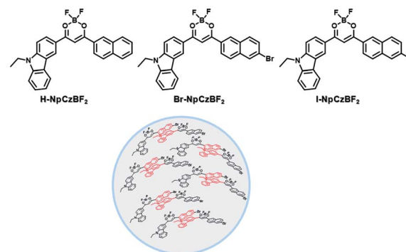
Fig. 18 Schematic illustration of the structures of the different substituents (H-NpCzBF 2 , Br-NpCzBF 2 , and I-NpCzBF 2 ) based on difluoroboron \beta -diketonate (BF 2 bdk) and carbazole.
