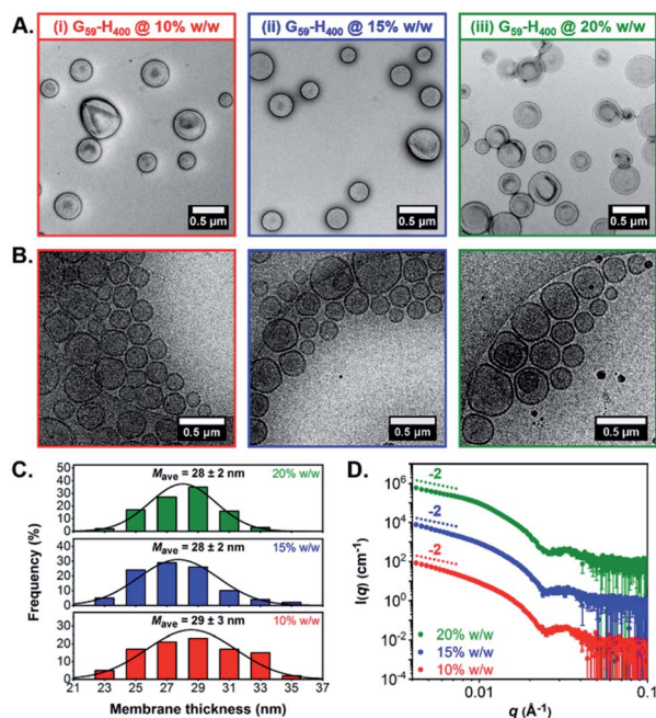
Fig. 1 Characterization of G_{59} -H 400 diblock copolymer precursor vesicles prepared via RAFT-mediated aqueous PISA when targeting (i) 10% w/w, (ii) 15% w/w or (iii) 20% w/w solids: (A) representative dry-state TEM images obtained using a 0.75% w/w uranyl formate staining solution; (B) corresponding representative cryo-TEM images; (C) membrane thickness distribution histograms and mean membrane thicknesses, determined by analyzing at least 100 vesicles in each case; (D) SAXS patterns recorded for 1.0% w/w aqueous vesicle dispersions.
