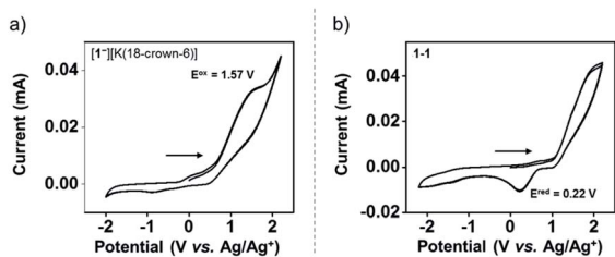
Fig. 4 Cyclic voltammetry (CV) of [1^-][K(18\text{-crown-6})] (9.3 mM) (a) and 1-1 (3.4 mM) (b) in dry 0.1 M [n\text{Bu}_4\text{N}][\text{ClO}_4]/\text{THF} solution obtained at 0.1\text{ V s}^{-1} scan rate using glassy carbon electrodes, Pt wire, and \text{Ag}/\text{Ag}^+ as the working, counter, and reference electrodes, respectively.
