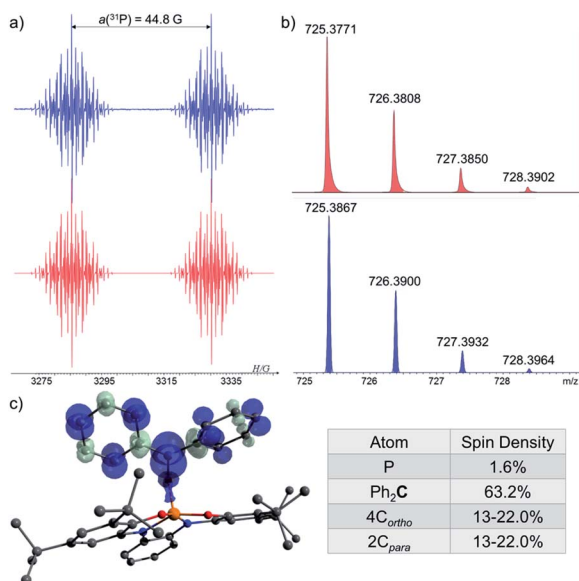
Fig. 6 (a) EPR spectra of [1\text{-OCPh}_2]^\bullet under UV-irradiation ( \lambda > 300 \text{ nm} ) at 370 K (blue), and its simulation (red); (b) MS of the reduced [1\text{-OCPh}_2]^\bullet (725.3771 (M) ^\bullet ) (red) and its simulation (blue); (c) DFT calculated Mulliken atomic spin densities in [1\text{-OCPh}_2]^\bullet .
