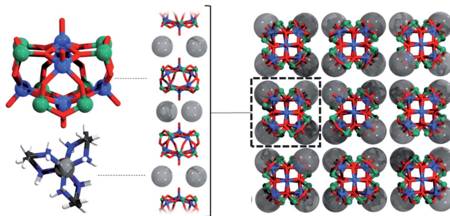
Fig. 3 Ball and stick representation of an individual [\text{V}_6\text{As}_8\text{O}_{26}]^{4-} polyanion and the [\text{Ni}(\text{en})_3]^{2+} dication (left), followed by their hierarchical packing from one (middle) to three dimensions (right). Colour code: V = blue, O = red, As = green, N = dark blue, Ni = grey, C = black, H = white spheres. For clarity, [\text{Ni}(\text{en})_3]^{2+} in the middle and right figure are represented as transparent grey spheres.
