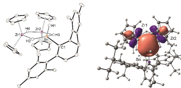
Fig. 4 ORTEP and NLMO exhibiting the three centre two electron bond of cation [(Cp_2ZrH)_2HSnHAR^+] of 10 . Thermal ellipsoids are shown at 50% probability level. Hydrogen atoms except the Zr–H and Sn–H units, methyl groups and the anion of 10 have been omitted. Selected interatomic distances [Å] and angles [ ^\circ ]: Zr1–Sn 3.0185(2), Zr2–Sn 3.0325(2), Zr1–Zr2 3.577(2), Zr1–Cp 2.4845(14) – 2.5328(15), Zr2–Cp 2.4760(14) – 2.5162(15), Sn–C1 2.1678(12), Sn–H1 1.57(3), Sn–H2 2.07(3), Sn–H3 1.98(3), Zr1–H2 1.84(3), Zr1–H4 2.00(2), Zr2–H3 1.89(3), Zr2–H4 1.97(2), Zr1–Sn–Zr2 72.5(1), C1–Sn–H1 95.8(10), H2–Sn–H3 144.7(11), H2–Zr1–H4 121.6(11), H3–Zr2–H4 118.3(10).
