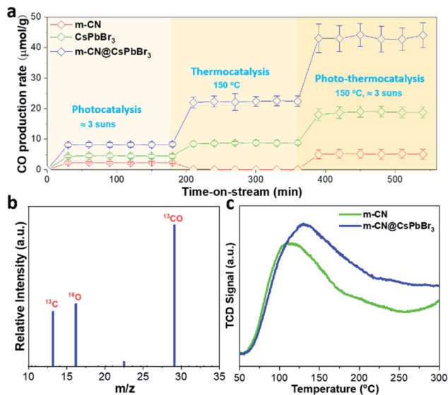
Fig. 3 (a) The CO 2 reduction to CO performance under the three conditions of photocatalysis, thermocatalysis and photo-thermocatalysis. For the latter two, the temperature is set to 150 °C; (b) mass spectrometry (MS) result of 13 CO produced over m-CN@CsPbBr 3 from the 13 CO 2 isotope experiment under thermocatalysis ( m/z , mass/charge ratio); (c) CO 2 -TPD results of the reference m-CN and the m-CN@CsPbBr 3 catalyst.
