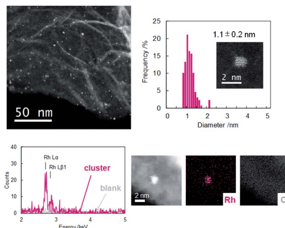
Fig. 2 STEM image, histogram, and EDX analysis of the synthesized Rh nanoparticle.
