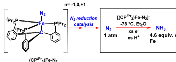
Fig. 30 Ammonia formation using a Fe–N 2 catalyst showing C atom as an anchor.
