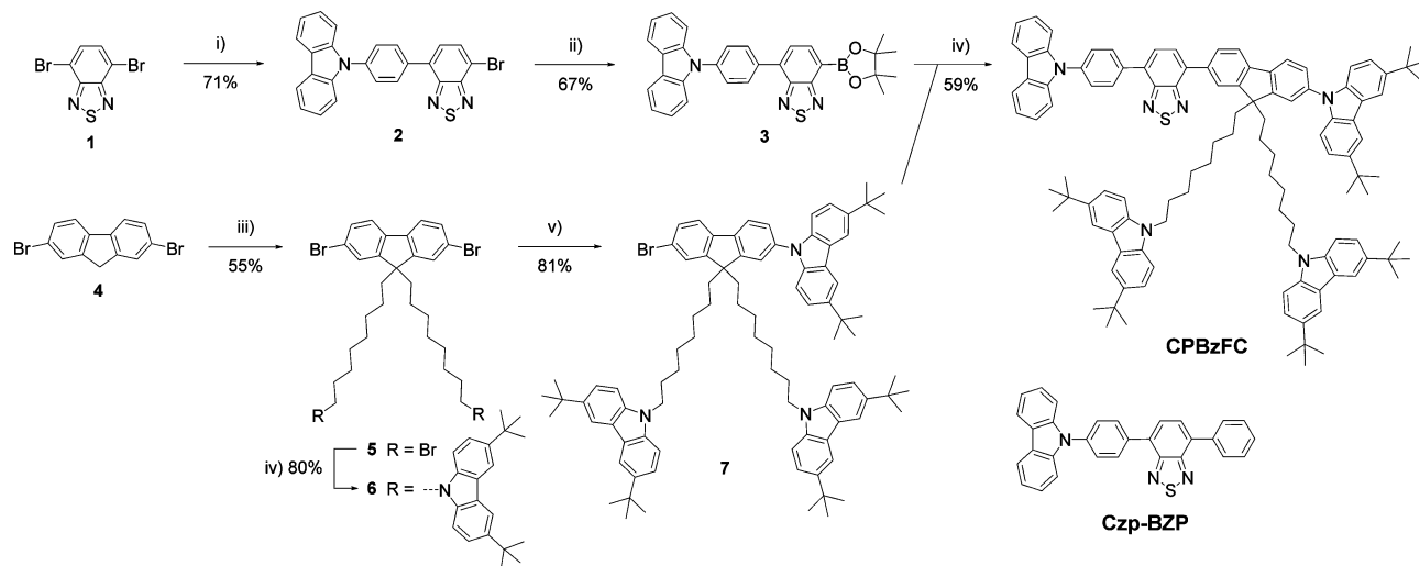
Scheme 1 Synthesis of CPBzFC . Reagents and conditions: (i) (4-(carbazol- N -yl)phenyl)boronic acid, Pd(PPh 3 ) 4 , 10% K 2 CO 3 (aq), THF, reflux; (ii) bispinacolatodiboron, KOAc, Pd(dppf) 2 Cl 2 , toluene, reflux; (iii) 1,8-dibromooctane, tert -BuNH 4 Br, KOH, DFM, H 2 O; (iv) 3,6-di- tert -butylcarbazole, KOH, DMF; (v) 3,6-di- tert -butylcarbazole, CuI, K 3 PO 4 , (±)- trans -1,2-diaminocyclohexane, toluene, reflux; (vi) Pd(PPh 3 ) 4 , 10% K 2 CO 3 (aq), THF, reflux.
