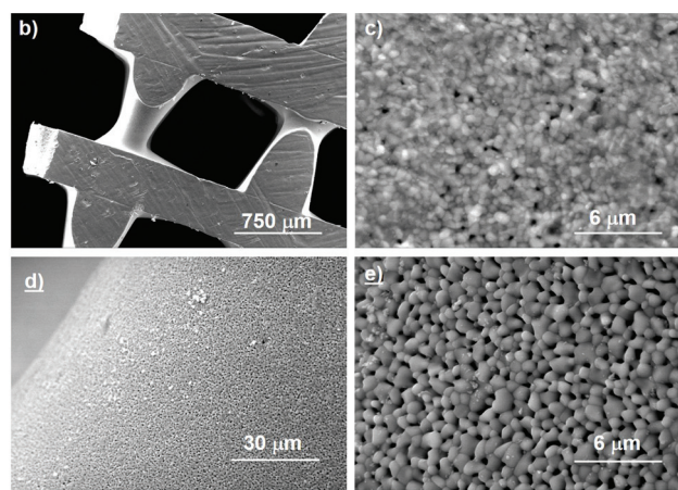
Fig. 3 XRD pattern of the ceria scaffold sintered at 1450 \text{ °C} , with the major peaks for cubic \text{CeO}_2 indexed. SEM images of a sintered and polished scaffold (b) show the interior (c) and exterior (d–e) microstructure.
