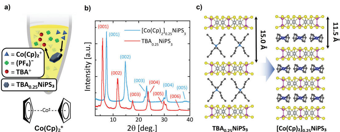
Fig. 2 (a) Setup for the cation exchange process. A \text{TBA}_{0.25}\text{NiPS}_3 bulk crystal is immersed in a closed vial containing an acetone nitrile solution of \text{Co}(\text{Cp})_2\text{PF}_6 . The chemical structure of bis-(cyclopentadienyl)cobalt(III), cobaltocenium ( \text{Co}(\text{Cp})_2^+ ) is also shown. (b) X-ray diffraction patterns of bulk \text{TBA}_{0.25}\text{NiPS}_3 before and after cation exchange (red and blue lines, respectively). Both patterns are normalized to the intensity of the (001) peak to facilitate their comparison. (c) Scheme of the cation exchange. During the process, the interlayer distance decreases from 15 Å to 11.5 Å due to the smaller size of \text{Co}(\text{Cp})_2^+ in comparison to \text{TBA}^+ .
