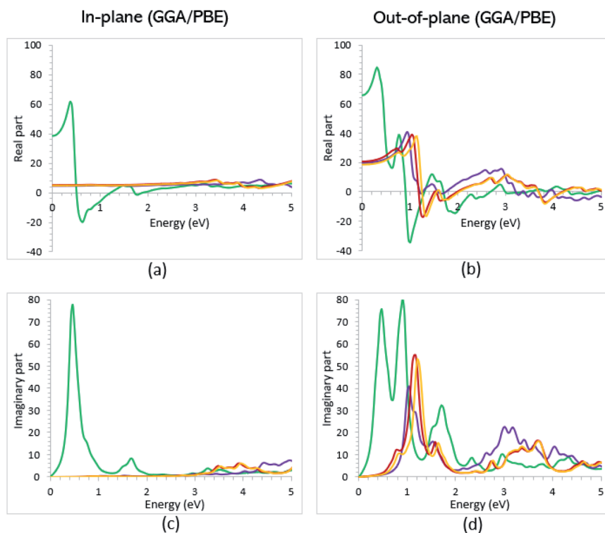
Fig. 4 Imaginary and real parts of the dielectric function of VO 2 (B) PP (green), VO 2 (B) LP (purple), VO 2 (B) PPD (red), and VO 2 (B) LPD (orange) structures along the in-plane (a and c) and out-of-plane (b and d) polarizations, as predicted by RPA + PBE.
