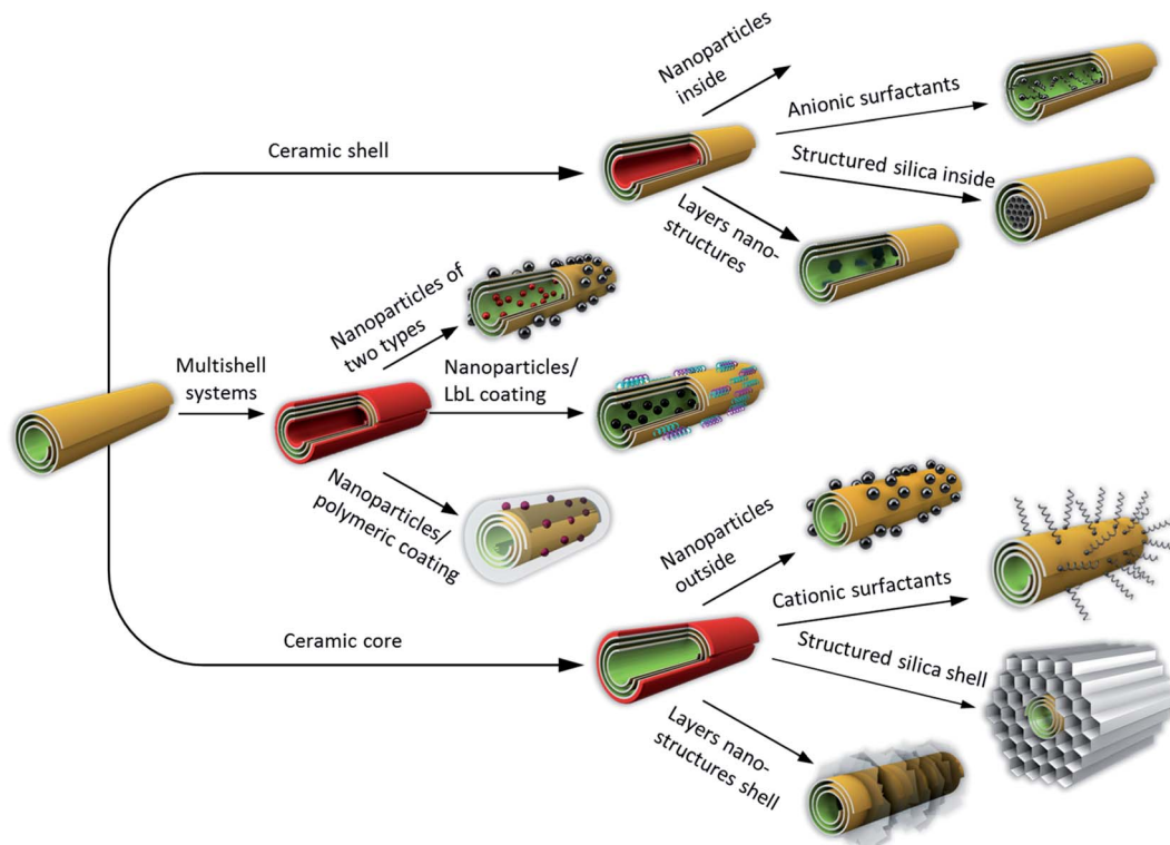
Scheme 1 Architectural approach in core-shell systems based on clay nanotubes' inside/outside modification with metal particles (round and platelets), outermost hydrophobization and mesosilica formation.
