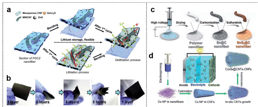
Fig. 2 Carbon-based foldable 1D electrode. (a) Schematic illustration of FGCZ structures and the mechanism for lithium storage. (b) Digital images of the multi-folded FGCZ film and the recovery state of the FGCZ film. Reproduced from ref. 43. Copyright 2019, Elsevier. (c) Schematic illustration of SnS 2 @CF by the electrospinning method. Reproduced from ref. 44. Copyright 2021, Royal Society of Chemistry. (d) Schematic illustration of the binder-free and free-standing Co 9 S 8 @CNT-CNF mats via the electrospinning method. Reproduced from ref. 45. Copyright 2018, Wiley-VCH.
