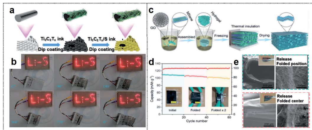
Fig. 5 MXene-based foldable 2D electrode. (a) Schematic illustration of the fabrication process of the MF@Ti 3 C 2 T x /S cathode. (b) A “Li–S” shaped string of light contains 30 LEDs lit by MF@Ti 3 C 2 T x /S50 electrode soft-packaged Li–S batteries at different bending angles. Reproduced from ref. 82. Copyright 2021, Royal Society of Chemistry. (c) Schematic illustration of the fabrication process of the MGA material. (d) Cycling performance of the LMO//MGA@Zn pouch cells at various folding times. (e) SEM images of the MGA sample after folding (left) and releasing (right) once (up) and twice (down). The inset images indicate the optical pictures of the MGA sample after folding once (up) and twice (down), respectively. Reproduced from ref. 83. Copyright 2021, Wiley-VCH.
