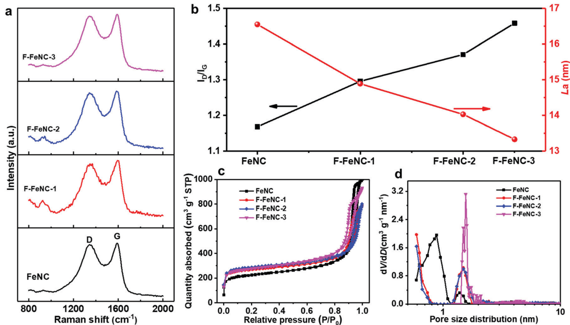
Fig. 2 (a) Raman spectra, (b) L_a sizes and the ratio of the G and D bands ( I_D/I_G ) in the Raman spectra, (c) \text{N}_2 adsorption/desorption isotherms and (d) pore size distributions processed from the non-local density functional theory (NLDFT) analysis FeNC, F-FeNC-1, F-FeNC-2, and F-FeNC-3.
