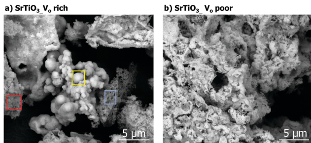
Fig. 5 SEM image of (a) V_O rich SrTiO_3 made with heating profile 1 and (b) V_O poor SrTiO_3 made with heating profile 2.
