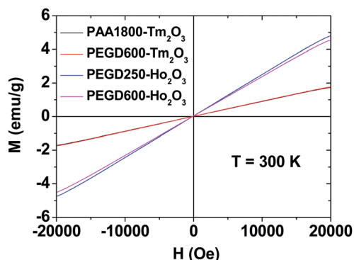
Fig. 7 Mass-corrected M-H curves of the PEGD250- and PEGD600-coated ultrasmall \text{Ho}_2\text{O}_3 nanoparticles, and PEGD600- and PAA1800-coated ultrasmall \text{Tm}_2\text{O}_3 nanoparticles at 300 K. The net M values of the ultrasmall \text{Ho}_2\text{O}_3 and \text{Tm}_2\text{O}_3 nanoparticles without ligands were used in the plots, which were estimated using the net masses of the nanoparticles extracted from the TGA curves.
