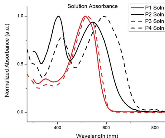
Fig. 1 Solution absorption profile of P1–P4 with the concentration of 10^{-5} M in chloroform.
