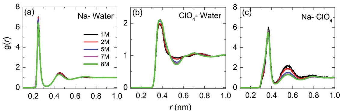
Fig. 5 Radial distribution functions for the center-of-mass for Na–water, ClO 4 –water and Na–ClO 4 as a function of the molar concentration.
