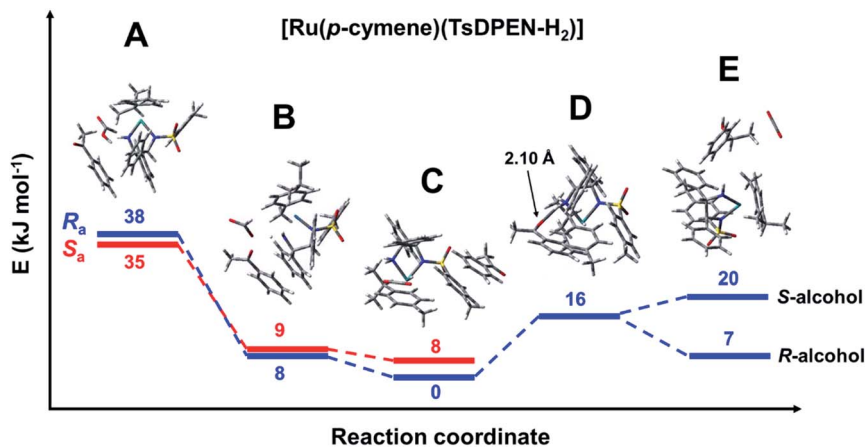
Fig. 5 Energy profile for the reduction of acetophenone catalysed by [\text{Ru}(p\text{-cymene})(\text{S},\text{S-TsDPEN-H}_2)] , with formic acid as the hydride donor. Note the axial chirality was taken into account only for the first three steps. Species A: [\text{Ru}(p\text{-cymene})(\text{S},\text{S-TsDPEN-H}_2)] + formic acid + acetophenone (Fig. S10 and S11, PDB7 and PDB8†). Species B: [\text{Ru}(p\text{-cymene})(\text{S},\text{S-TsDPEN-H})]^+ + formate + acetophenone (the white dot in the middle is showing the transfer of \text{H}^+ ), Fig. S12 and S13, PDB9 and PDB10.† Species C: [\text{R-Ru}(p\text{-cymene})(\text{S},\text{S-TsDPEN-H})\text{H}] + \text{CO}_2 + acetophenone (Fig. S2 and S9: PDB6, Fig. S14 and S15: PDB11 and PDB12†). Species D: [\text{R-Ru}(p\text{-cymene})(\text{S},\text{S-TsDPEN-H-acetophenone})\text{H}] + \text{CO}_2 (Fig. S16, PDB13†) Species E: [\text{Ru}(p\text{-cymene})(\text{S},\text{S-TsDPEN-H}_2)] + \text{CO}_2 + phenylethanol (Fig. S17 and S18, PDB14 and PDB15†). Note, bonds between Ru and p -cymene are omitted for clarity.
