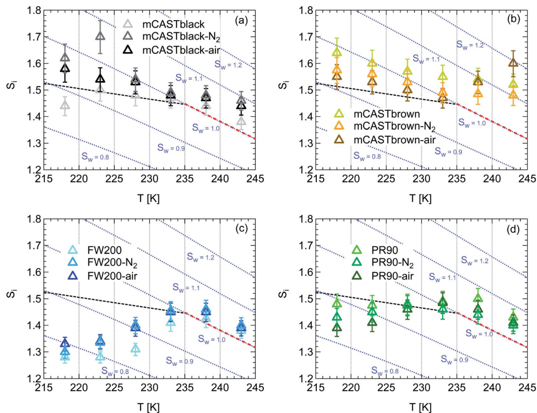
Fig. 3 Onset (at \text{AF} = 0.1\% ) ice saturation ratio ( S_i ) as a function of T for fresh and denuded 200 nm mCASTblack (a), mCASTbrown (b), FW200 (c) and PR90 (d). AF is reported from the 1.0 \mu\text{m} OPC channel. Black dashed line: homogeneous freezing conditions for solution droplets at T < \text{HNT} , according to Koop et al. 45 Light blue dotted line: constant water saturation conditions calculated based on Murphy and Koop. 44 Red dashed line: the 1.0 \mu\text{m} size water droplet survival conditions for T > \text{HNT} , where the phase of the particle larger than 1.0 \mu\text{m} can be either ice or liquid water. The S_i uncertainty due to the temperature uncertainty ( \pm 0.1 \text{ K} ) of the HINC chamber is indicated as error bars. Each data point was derived from the AF curves in Fig. 13–16 presented in the Appendix in which each AF curve is an average of at least two individual RH ramps.
