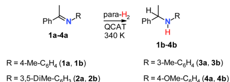
Scheme 2 The studied imine hydrogenations.
