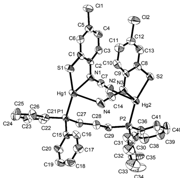
Fig. 5 Molecular structure of [\text{Hg}\{\text{SC}_6\text{H}_3\text{CIN}(\text{C}\equiv\text{N})\}_2(\mu\text{-dppb})] ( 8c ). Thermal ellipsoids at the 50% level and hydrogen atoms are omitted for clarity. Selected bond lengths (Å) and bond angles ( ^\circ ): Hg1–N1 2.367(6), Hg1–N4 2.835(6), Hg2–N2 2.723(6), Hg2–N3 2.249(8), Hg1–S1 2.372(2), Hg2–S2 2.372(2), Hg1–P1 2.395(2), Hg2–P2 2.385(2), Hg1...Hg2 5.481(2), N1–C7 1.312(11), N2–C7 1.149(11), N3–C14 1.280(12), N4–C14 1.173(12); N1–Hg1–S1 81.06(18)^\circ , N1–Hg1–P1 114.72(18)^\circ , S1–Hg1–P1 157.36(8)^\circ , N3–Hg2–S2 81.6(2)^\circ , N3–Hg2–P2 122.5(2)^\circ , S2–Hg2–P2 155.74(8)^\circ .
