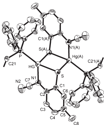
Fig. 4 Molecular structure of [Hg(SC 6 H 3 MeN(C≡N))(DMF)(μ-κ 1 ,κ 1 -dppe)] n (7b). Thermal ellipsoids at the 50% level and hydrogen atoms omitted for clarity and disordered DMF are omitted for clarity. Selected bond lengths (Å) and bond angles (°): Hg–N1 2.275(3), Hg–S 2.4370(9), Hg(A)–S 2.9350(9), Hg–O 2.880(5), Hg–S–Hg(A) 87.12 (3), N1–Hg–P 128.61(9), N1–Hg–S 81.13(9), S–Hg–P 146.39(3), S(A)–Hg–S 92.88(3), S(A)–Hg–P 102.32(3). Symmetry operator A: 1 – x, 1 – y, 1 – z.
